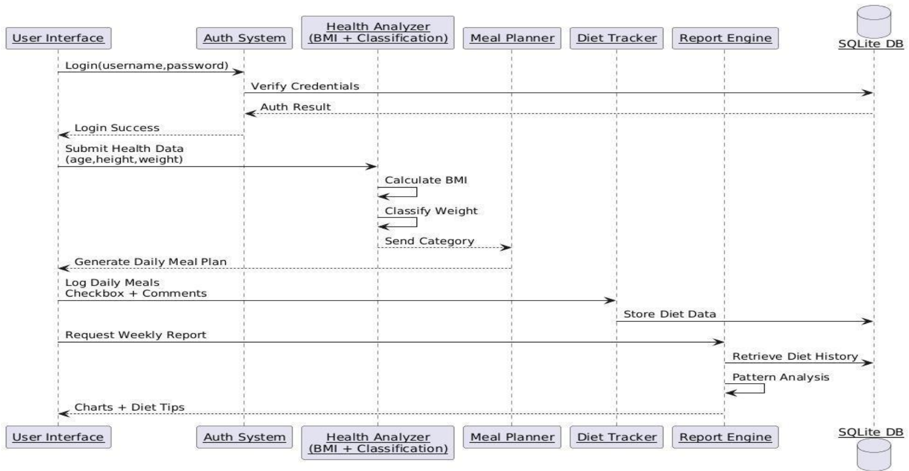
EAT-SMART Sequence Diagram
