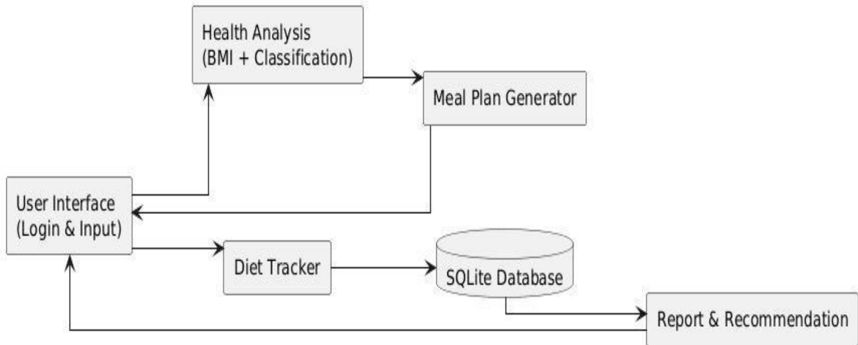
EAT-SMART Data Flow Diagram
